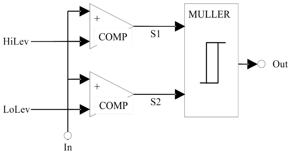
Figure 4 - The hysteresis comparator
