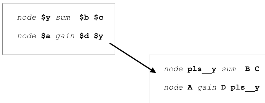
Figure 9 - The parsing mechanism of a cell (b)
