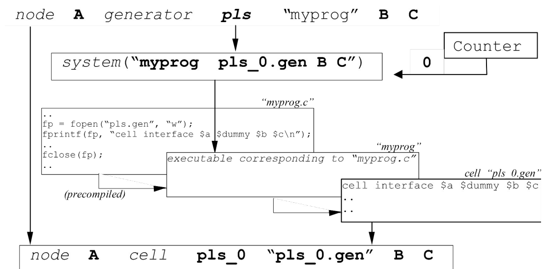
Figure 16 - The parameters of a generator
