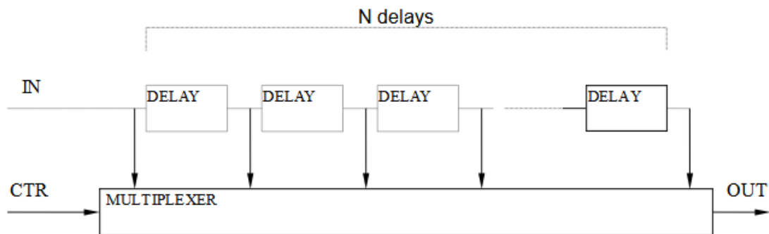
Figure 15 - Programmable delays
