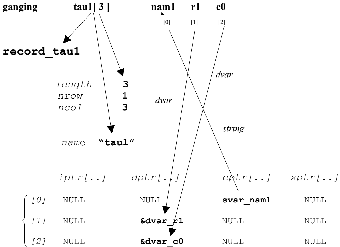
Figure 23 - How NAPA variables are passed by addresses
