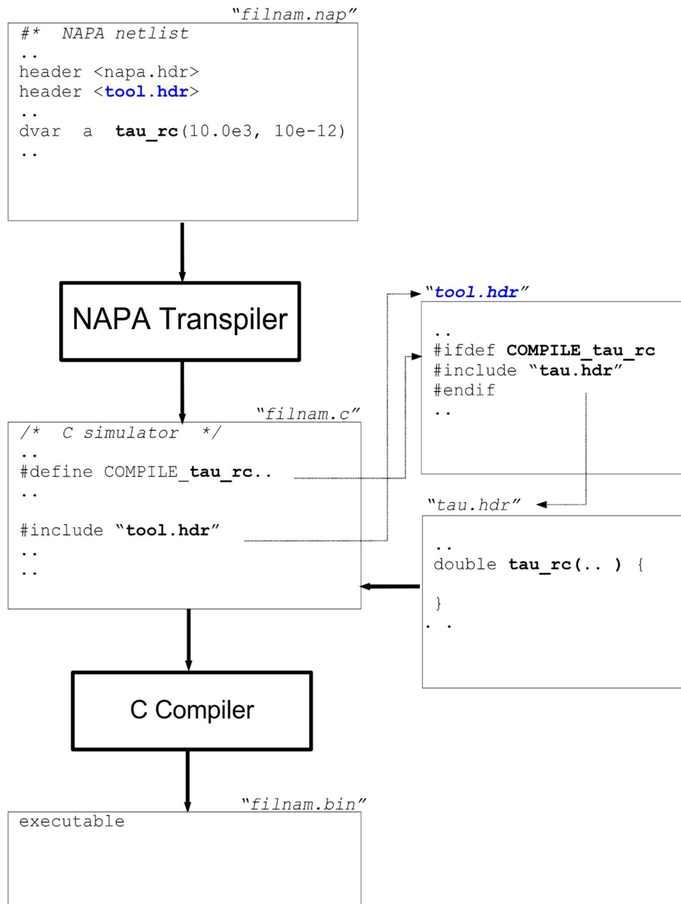
Figure 17 - The C macro preprocessor and the functions
