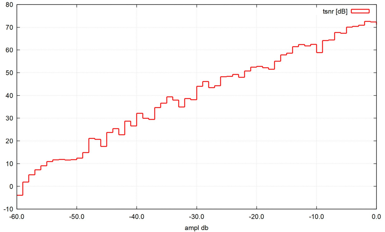
SIGMA-DELTA MODULATOR (MASH 2) analyzed at frequency 1.00 k Hz
